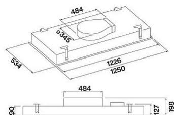
Hood and motor dimensions
